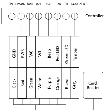
Figure 3-4 Wiring for Wiegand Communication Mode
