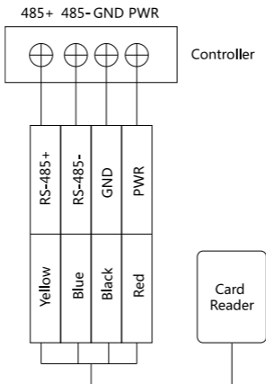
Figure 3-3 Wiring for RS-485 Communication Mode
