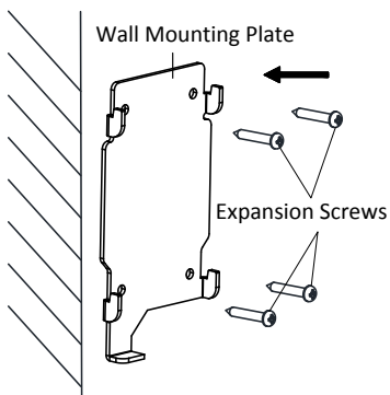
Figure 4-2 Install the Plate
