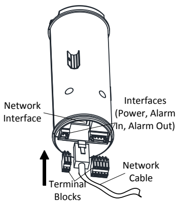
Figure 4-3 Insert Terminals and Network Cable
