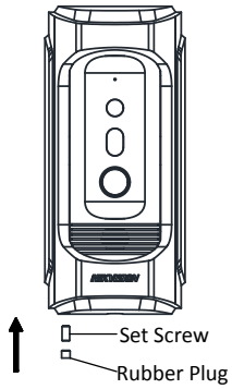
Figure 4-6 Secure the Door Station
