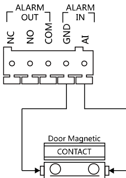
Figure 3-3 Door Magnetic Wiring
