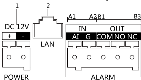
Figure 3-1 Terminals and Interfaces
