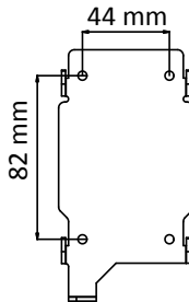
Figure 4-1 Wall Mounting Plate
