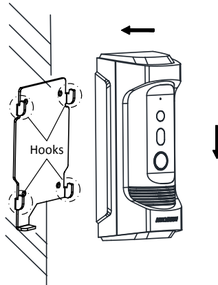
Figure 4-5 Hook the Door Station to the Plate
