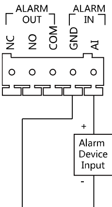
Figure 3-5 Alarm Device Input Wiring
