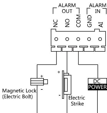
Figure 3-2 Door Lock Wiring
